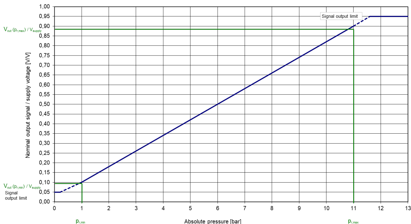
Output signal @ T_o = 25\text{ °C} , V_{\text{supply}} = 5\text{ V}
