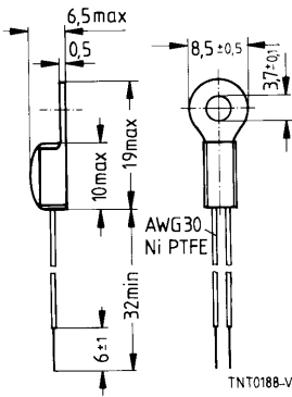
Dimensions in mm Approx. weight 0,8 g
