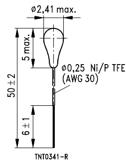
Dimensions in mm Approx. weight 60 mg
