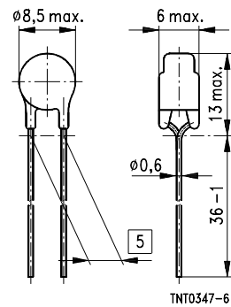
Dimensions in mm Approx. weight 0,6 g
