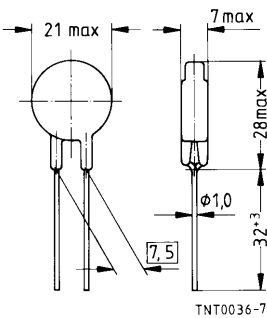
Dimensions in mm Approx. weight 4 g
