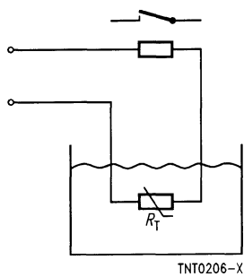
Figure 15 Circuit for liquid level sensing
