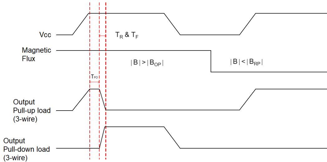
Power-On Output Waveform
