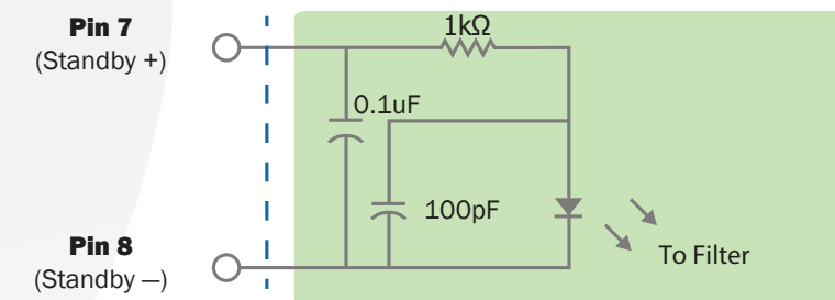
Figure C: An equivalent circuit looking into the STANDBY pin.
