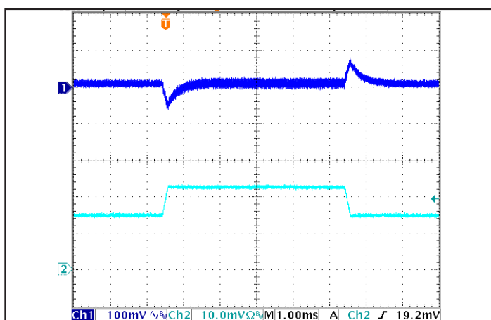
Figure 5: Output voltage response to step-change in load current (50 % -75 % -50 % of I out (max); dI/dt = 0.1 A/μs). Load cap: 1 μF ceramic and 15 μF tantalum capacitors. Ch 1: V out (100 mV/div), Ch 2: I out (20 A/div).
