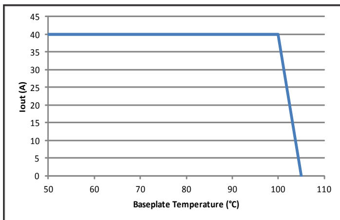
Figure 3: Maximum load current vs. baseplate temperature when conductively cooled. Note: The system design must provide a suitable thermal path that maintains the baseplate temperature below 100 °C (nominal input voltage).
