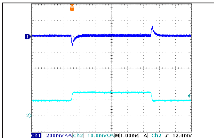
Figure 5: Output voltage response to step-change in load current (50 % -75 % -50 % of I out (max); dI/dt = 0.1 A/μs). Load cap: 1 μF ceramic and 15 μF tantalum capacitors. Ch 1: V out (200 mV/div), Ch 2: I out (20 A/div).
