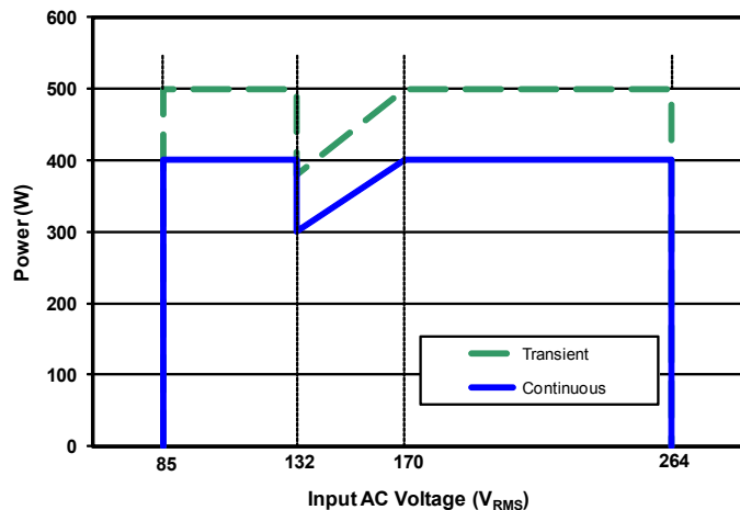
Figure 10: Rated output power vs Input AC Voltage
