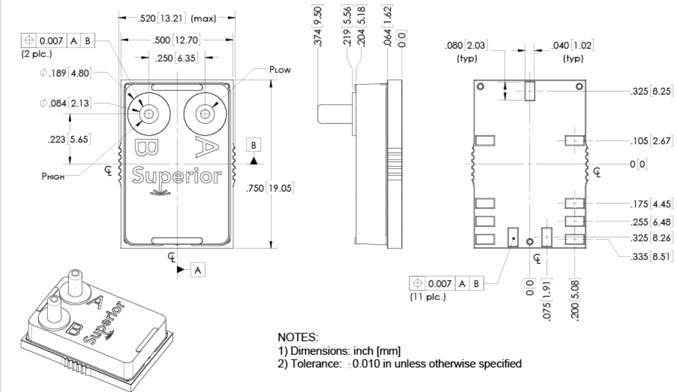
SM02 Package Dimensions
