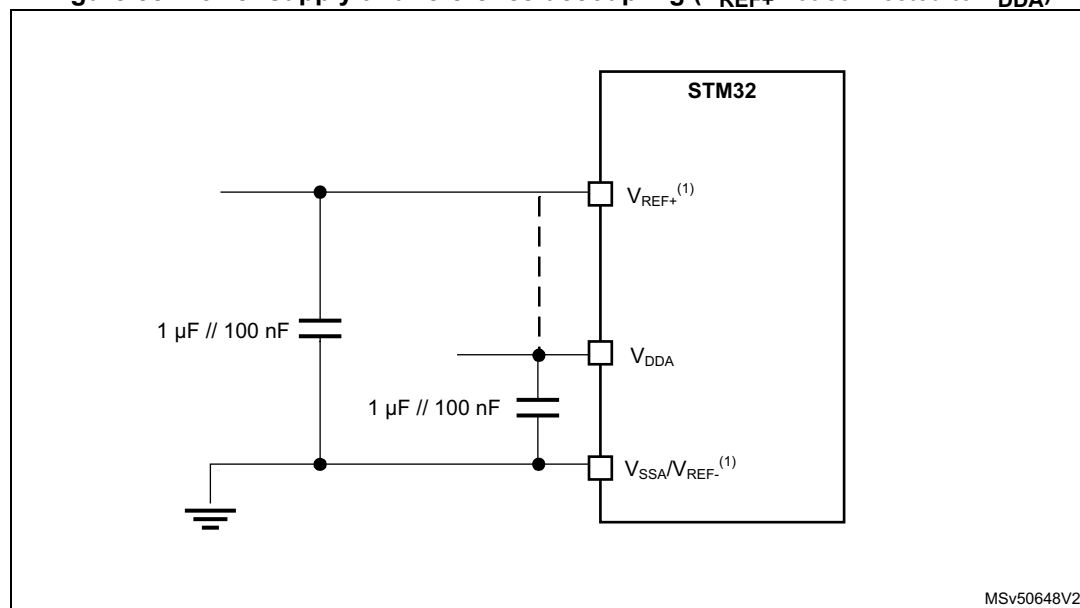
Figure 58. Power supply and reference decoupling ( V_{\text{REF+}} not connected to V_{\text{DDA}} )
