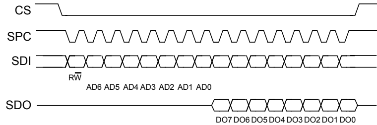
Figure 12. SPI read protocol (in mode 3)
