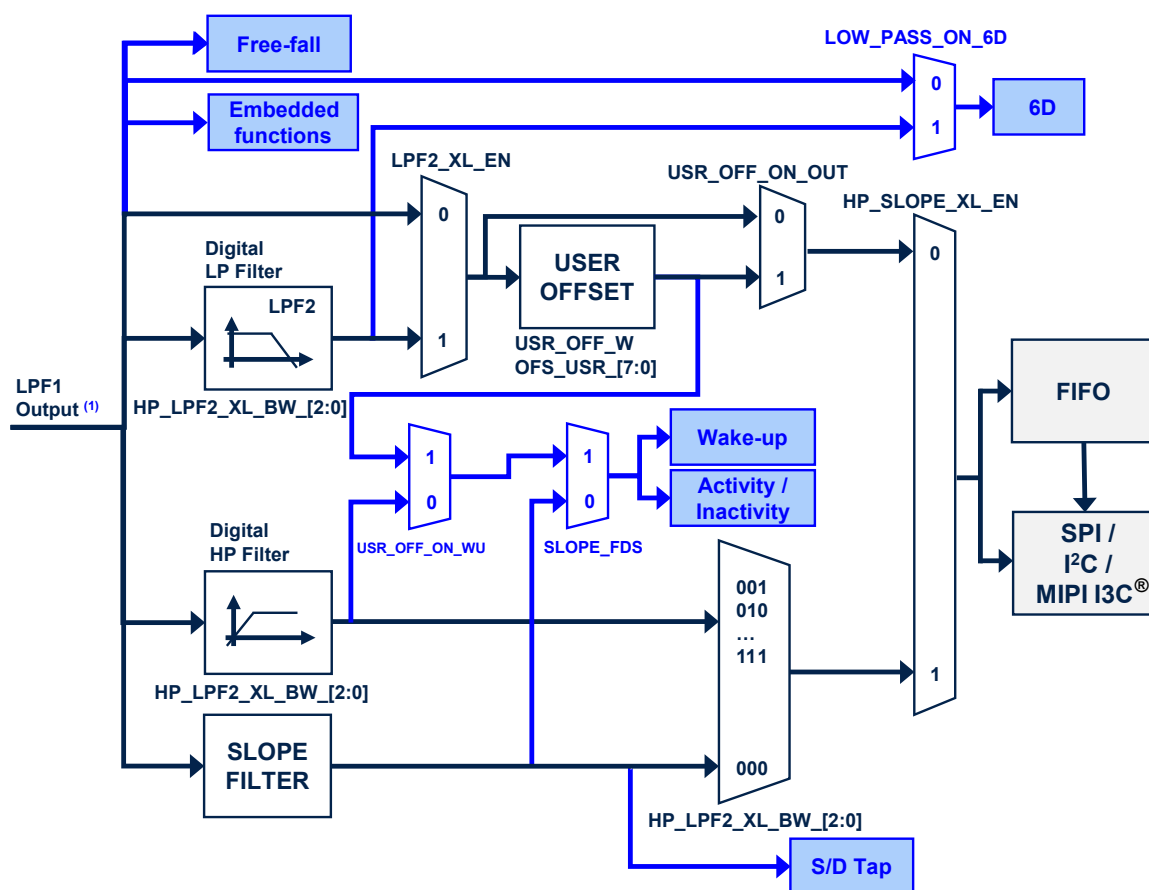
Figure 6. Accelerometer composite filter
