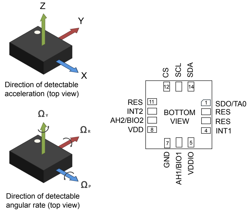
Figure 1. Pin connections
