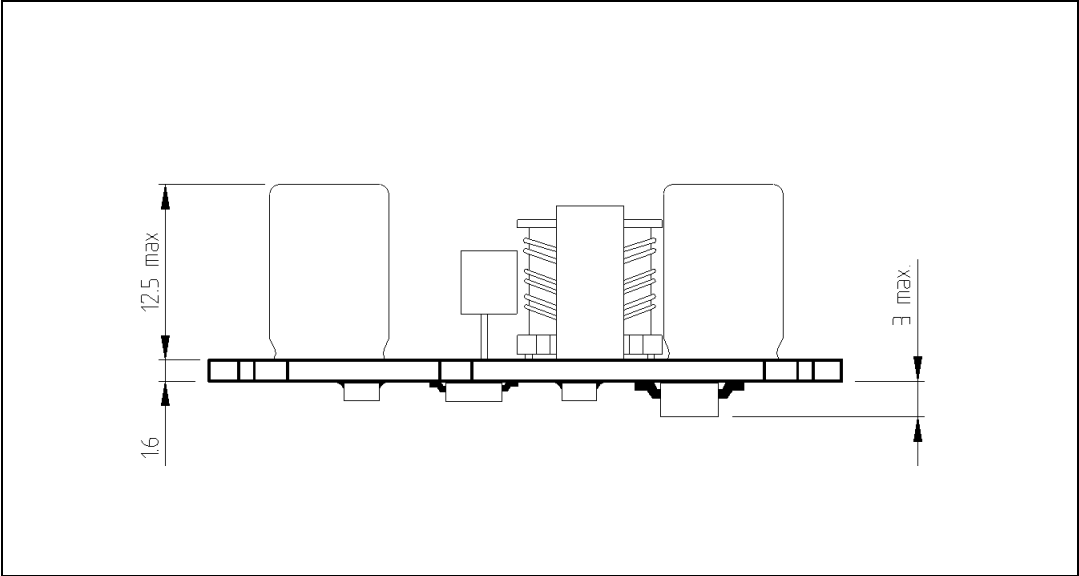
Figure 4. SPDC400FC mechanical data side view (dimensions in mm)
