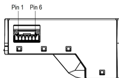
Figure 4 Pin layout. The communication interface connector (ACES 51451-0060N-001) is located at the side of the sensor adjacent to the air outlet.
