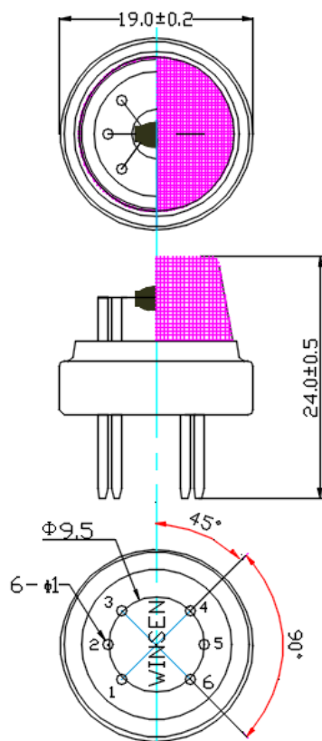
Fig1.Sensor Structure
