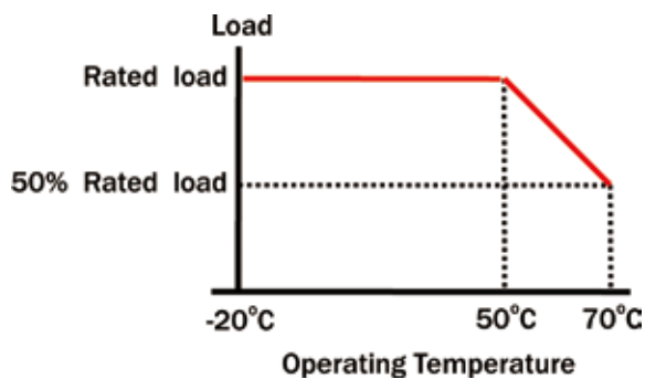
11. Power derating curve
