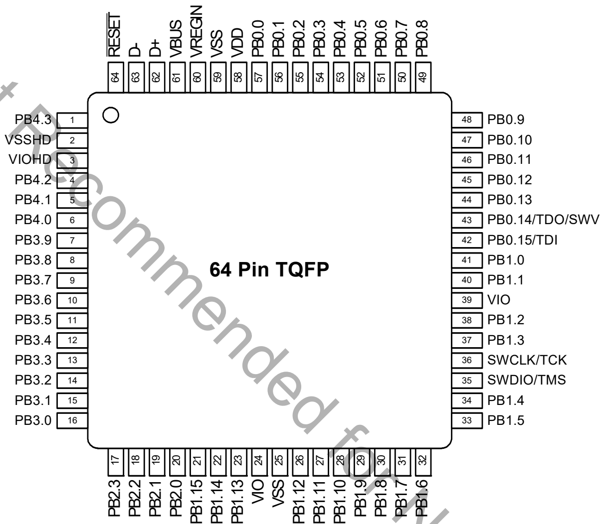
Figure 6.3. SiM3U1x6-GQ Pinout
