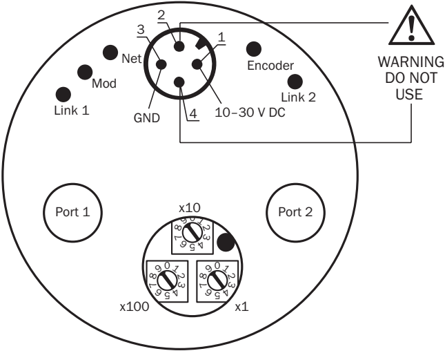
Connection diagram
