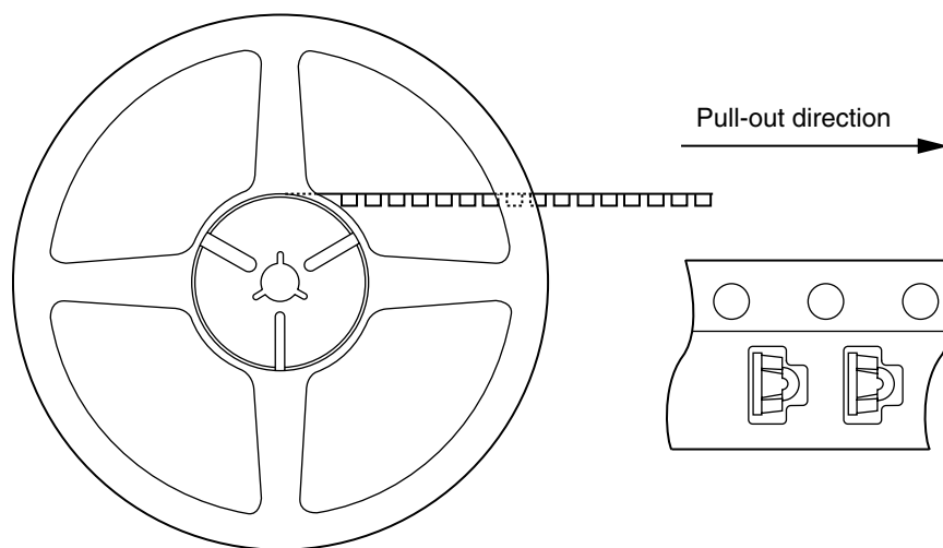
Fig. 7 Product Insertion Direction
