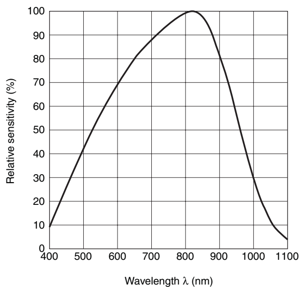
Fig. 2 Spectral Sensitivity (TYP.)
