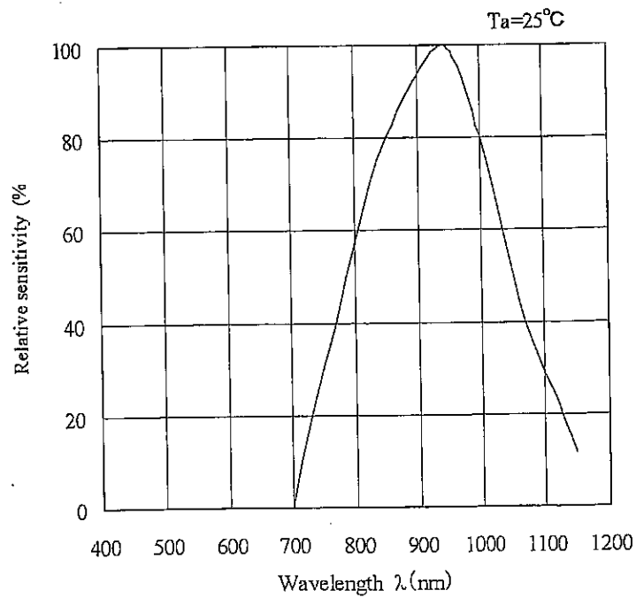
(Fig.6) Spectral sensitivity (TYP)
