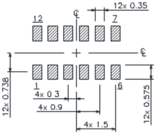
Recommended PCB PAD Layout
