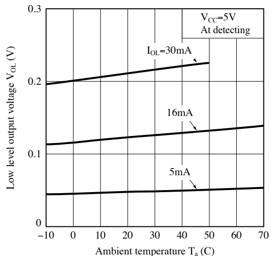
Fig.6 Low Level Output Voltage vs. Ambient Temperature
