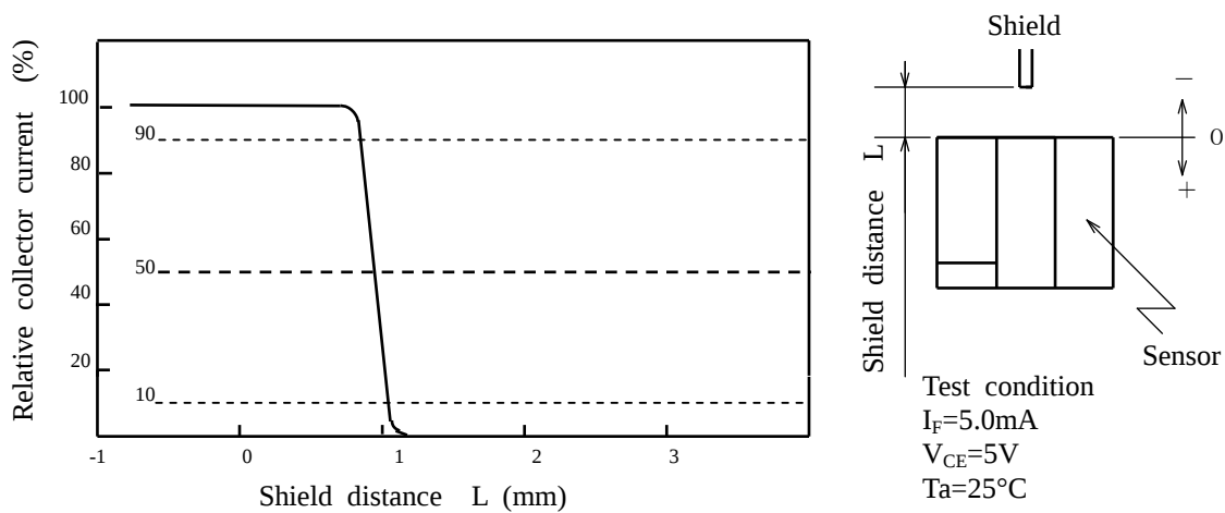
Relative collector current vs. shield distance 1 (Reference value)
