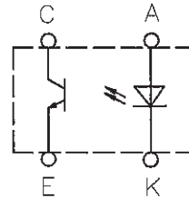
Circuit:Top View
