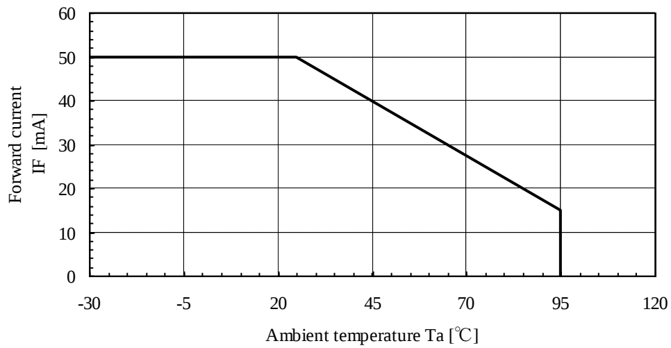
Fig.1 Forward current vs. ambient temperature
