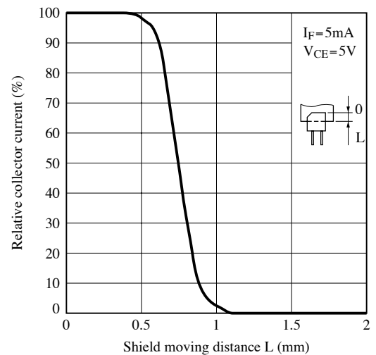
Fig.12 Detecting Position Characteristics (2)
