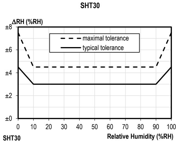
Figure 2 Tolerance of RH at 25°C for SHT30
