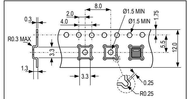
Figure 14 Sketch of packaging tape and sensor orientation. Header tape is to the right and trailer tape to the left on this sketch.
