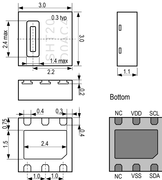
Figure 1: Drawing of SHT20P sensor package, dimensions are given in mm (1mm = 0.039inch), tolerances are \pm 0.1 mm. The die pad (center pad) is internally connected to VSS. The NC pads must be left floating. Numbering of E/O pads starts at lower right corner (indicated by notch in die pad) and goes clockwise (compare Table 2).
