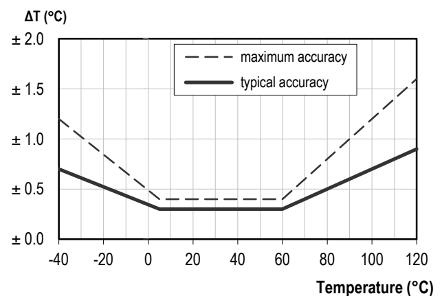
Figure 3 Typical and maximal temperature accuracy tolerance
