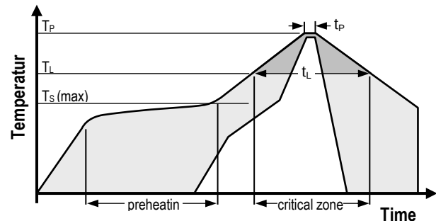
Figure 9 Soldering profile according to JEDEC standard. T_P \leq 260^\circ\text{C} and t_P < 30 sec for Pb-free assembly. T_L < 220^\circ\text{C} and t_L < 150 sec. Ramp-up/down speeds shall be < 5^\circ\text{C/sec} .
