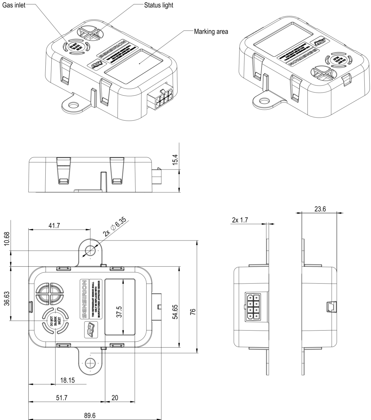
Figure 3: Physical dimensions of the SGD43S-M3-Sx in mm. Tolerances according to DIN ISO 2768-c.
