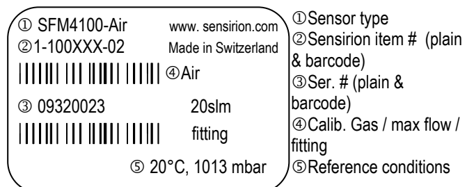
Figure 5: Label sticking on each sensor
