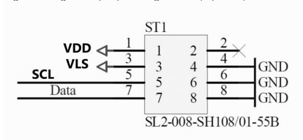
Figure 4: Digital output pin assignments (top view)
