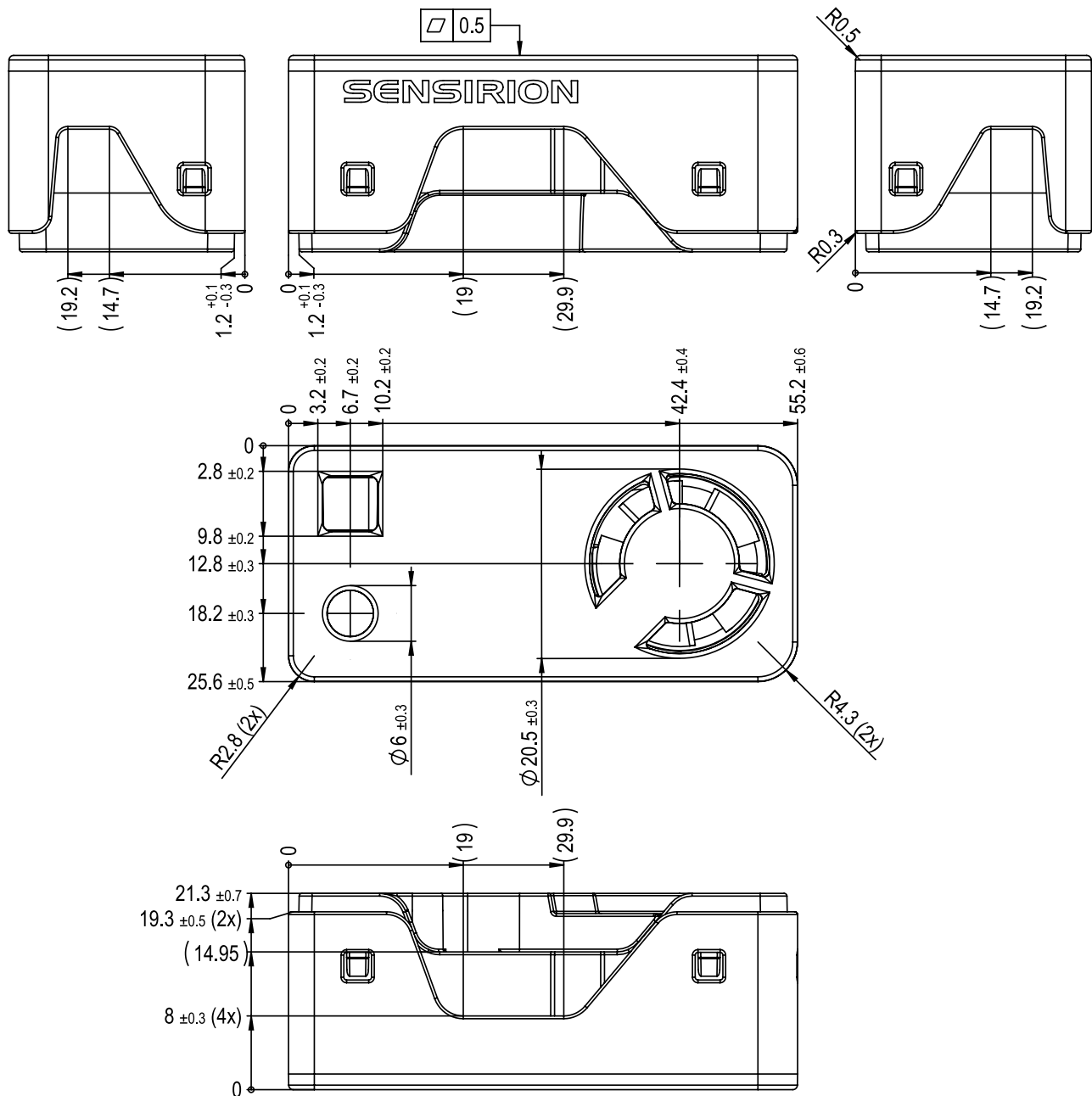
Figure 10. Technical Drawing of the SEN6x platform
