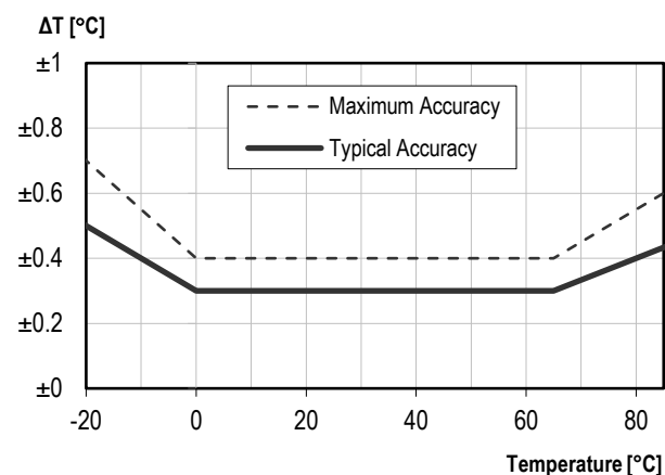
Figure 3 Temperature Accuracy Specification
