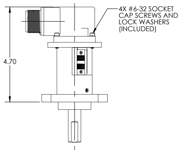
11008-003 HIGH-LOAD BEARING ASSEMBLY FOR H20D (SOLD SEPARATELY)
