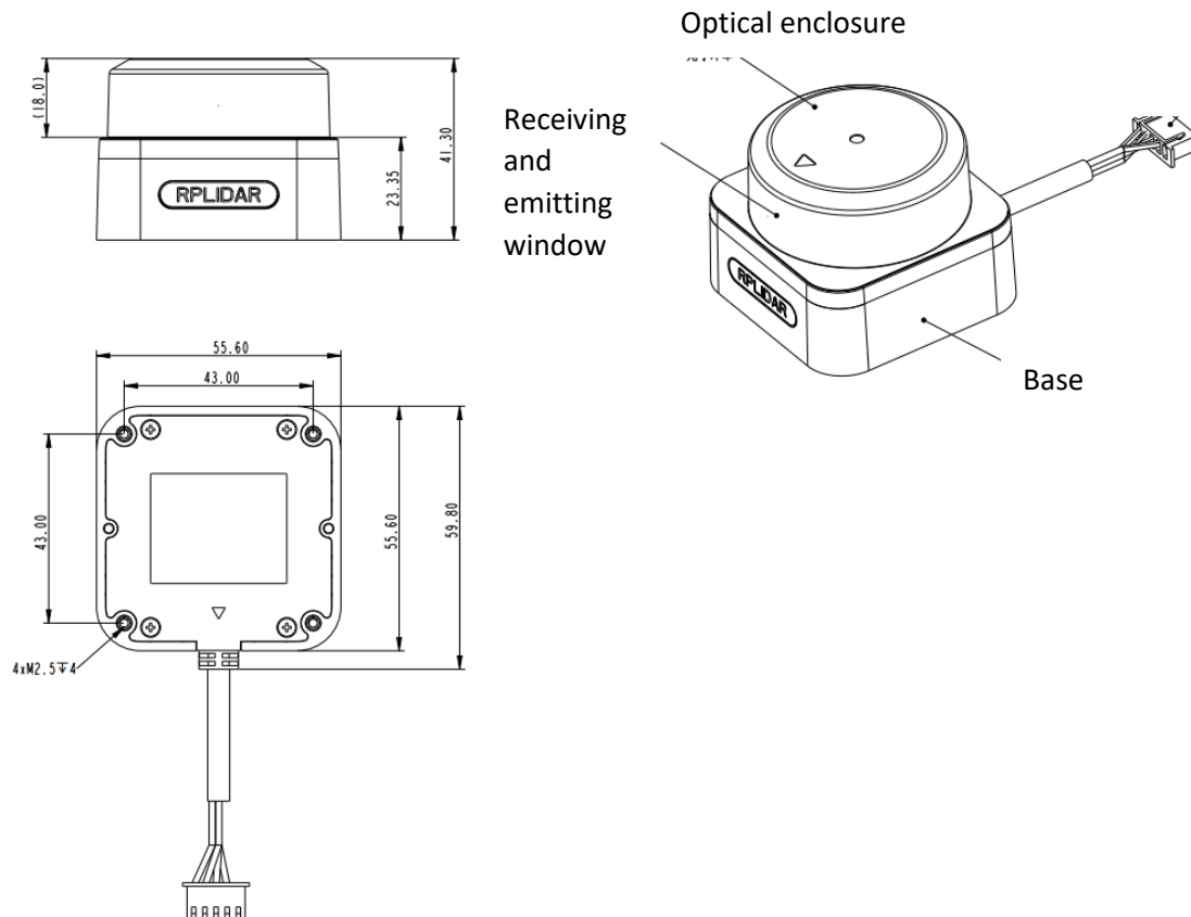
Figure 4-1 RPLIDAR S3 Mechanical Dimensions
