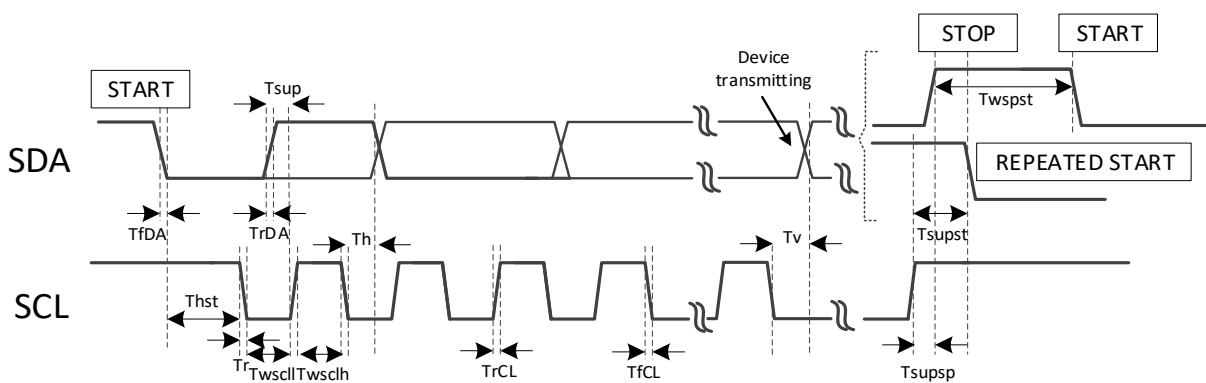
Figure 18: I²C timing diagram
