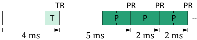
Figure 8: Typical timings for a continuous pressure-only measurement ( \text{MEAS\_T} = 0 , \text{P\_CONV} = 0 ) with activated 2× oversampling ( \text{OVSP} = 1 )
