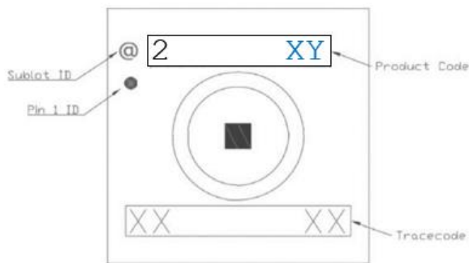
Figure 20: ENS21x marking
