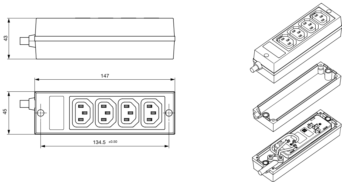
Mounting holes for 3 mm screws, with 2 meter cable and appropriate plug
