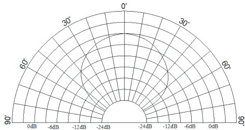
Directivity
