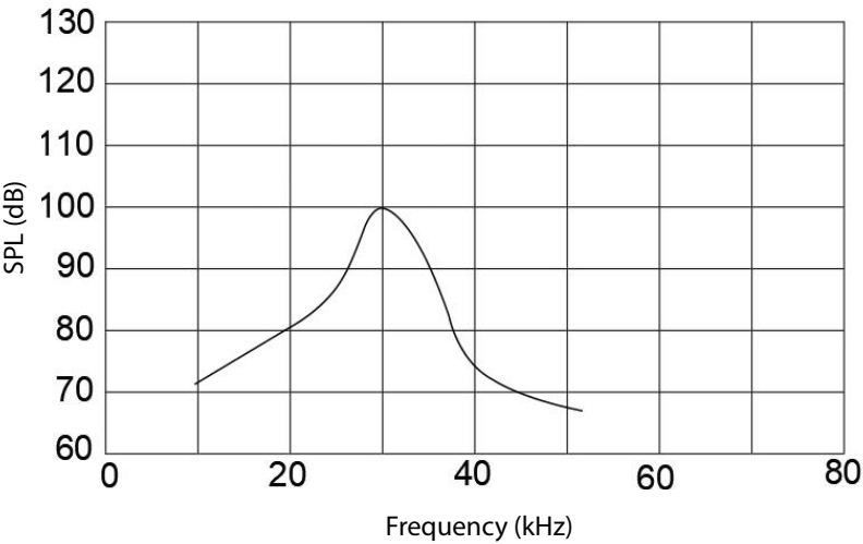
SPL vs. Frequency
