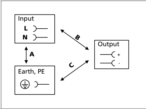
Fig. 17-1 Dielectric strength
