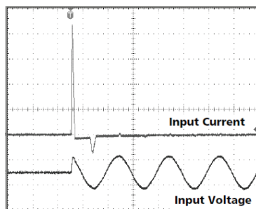
Fig 5-1 Input inrush current, typical behavior
