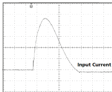
Fig 5-2 Input inrush current, zoom into first peak
