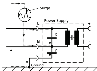
Fig. 20-3 Earthed input
