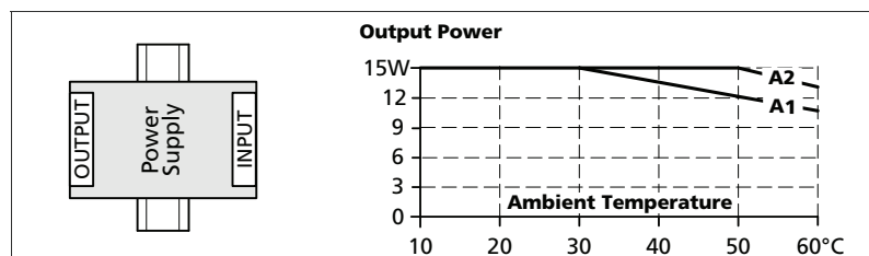
Fig. 20-9 Mounting Orientation E (Horizontal ccw)
