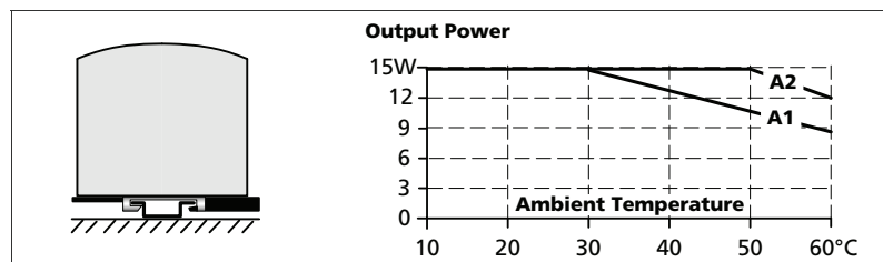
Fig. 20-7 Mounting Orientation C (Table-top mounting)
