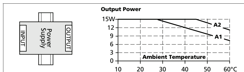
Fig. 20-8 Mounting Orientation D (Horizontal cw)
