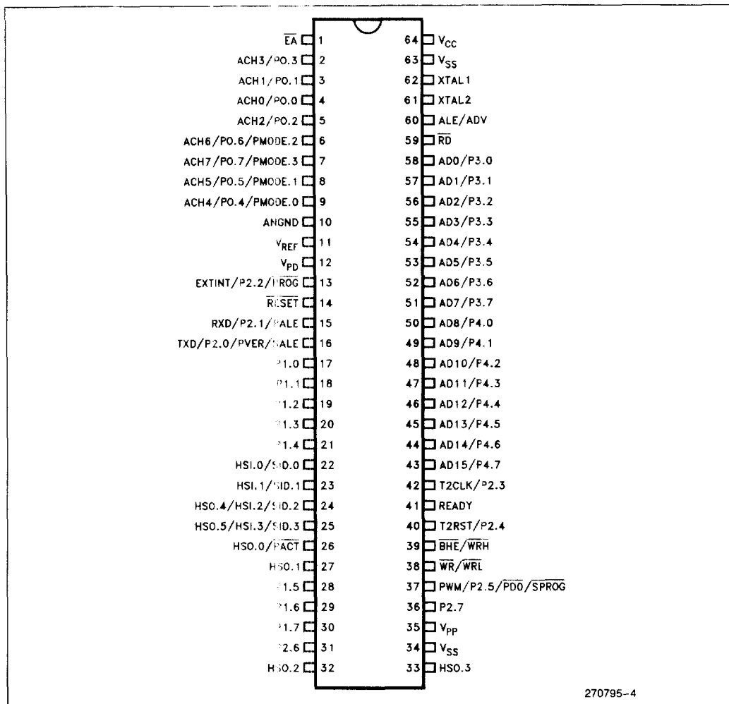
Figure 6. Shrink-DIP Package
