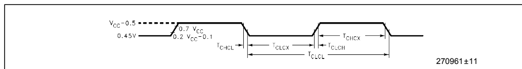
Figure 10. Clock Signal Waveform for I_{CC} Tests in Active and Idle Modes. T_{CHCX} = T_{CHCL} = 5 ns.
