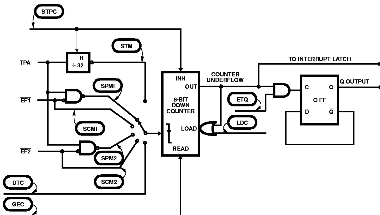
FIGURE 7. TIMER/COUNTER DIAGRAM
