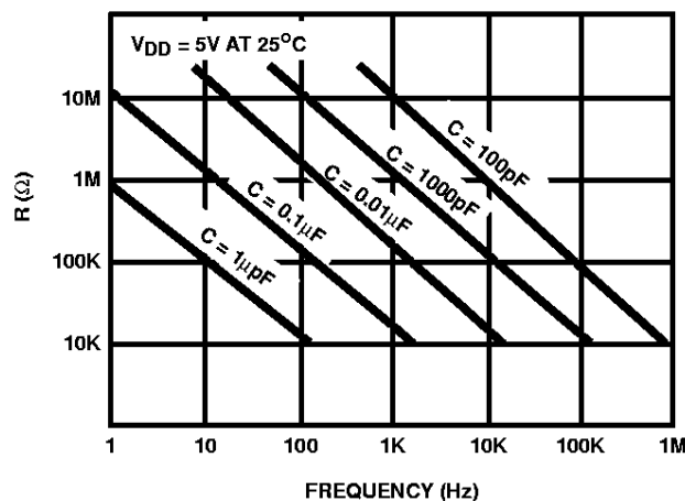
FIGURE 10. NOMINAL COMPONENT VALUES AS A FUNCTION OF FREQUENCY FOR THE RC OSCILLATOR
