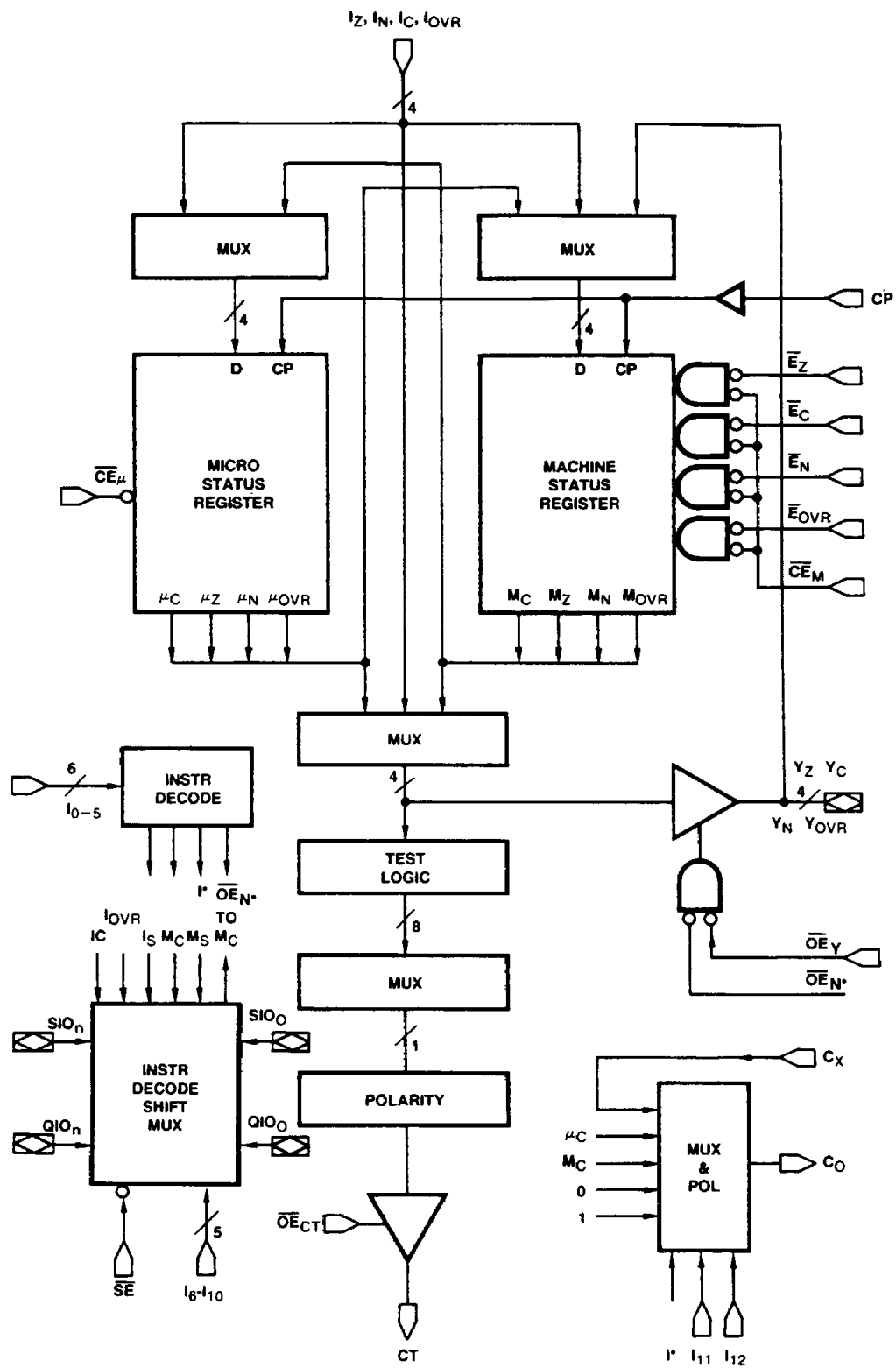
Figure 1. Detailed Block Diagram
