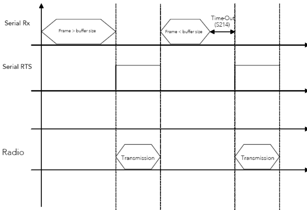
Figure 5-1: Flow Control Timing Diagram
