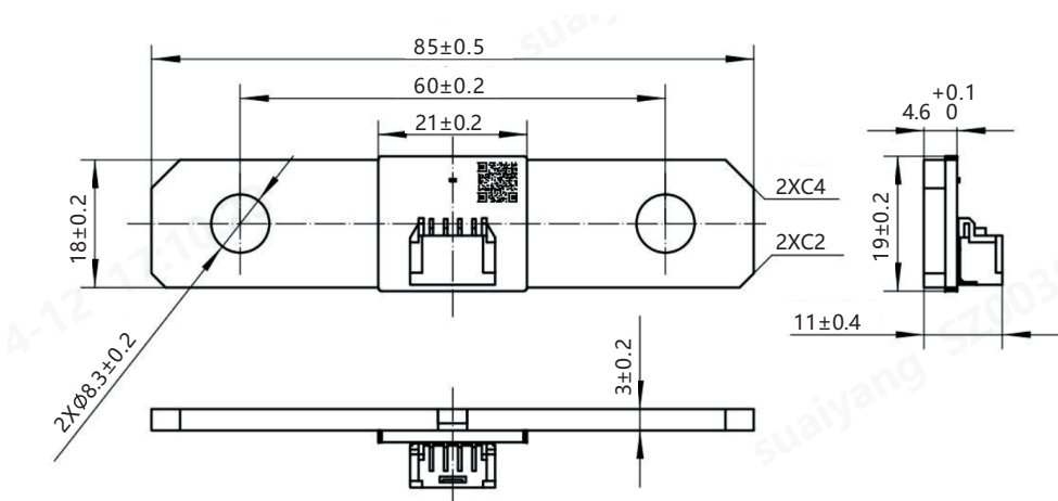
Figure 8. 1 Structure Diagram
