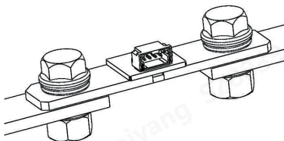
Figure 8-2. 8518 Shunt Connection Diagram
