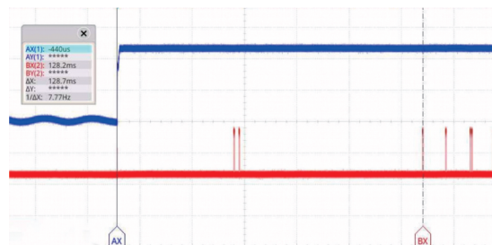
Figure 5-6 Sample6 Start-Up Time Test Curve
