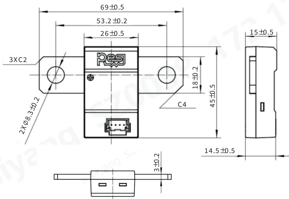
Figure 8.1 Structure Diagram
