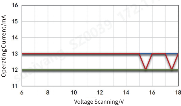
Figure 5-9 -40°C Current Consumption Test Curve
