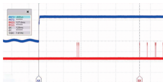
Figure 5-8 Sample8 Start-Up Time Test Curve
