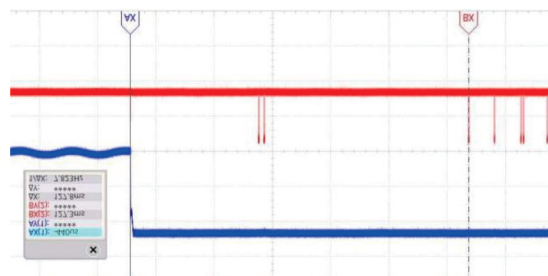
Figure 5-2 Sample2 Start-Up Time Test Curve
