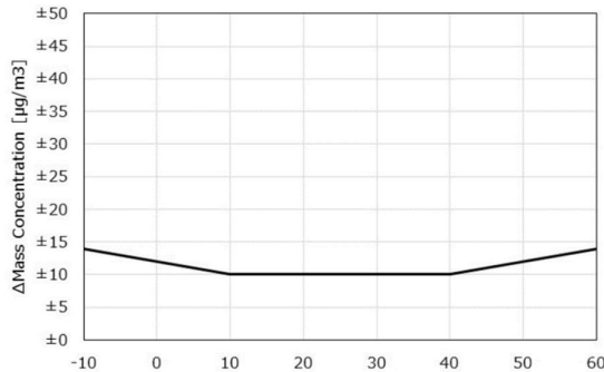
Figure 4. Consistency vs. Temperature (PM1_2: 0 - 100 \mu\text{g}/\text{m}^3 )
