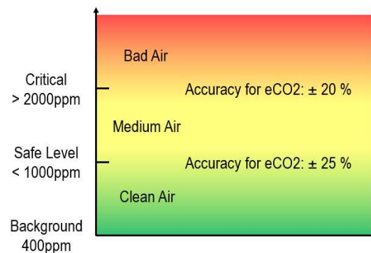
Figure 9. Concentration Dependent Accuracy for eCO 2
