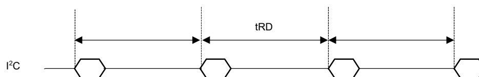
Figure 18. I²C Data Access Period
