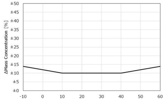
Figure 5. Consistency vs. Temperature (PM1_2: 100 - 500 \mu\text{g}/\text{m}^3 )
