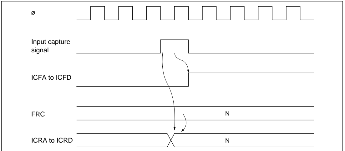
Figure 9.28 ICFA to ICFD Set Timing
