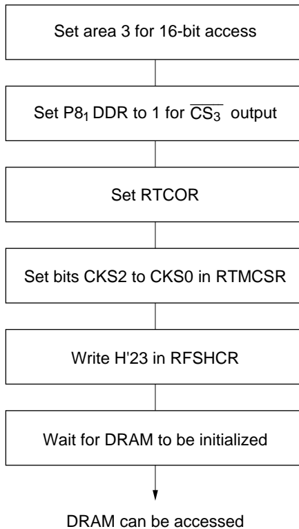
Figure 7-8 Setup Procedure for 2WE 1-Mbit DRAM (1-Mbyte Mode)
