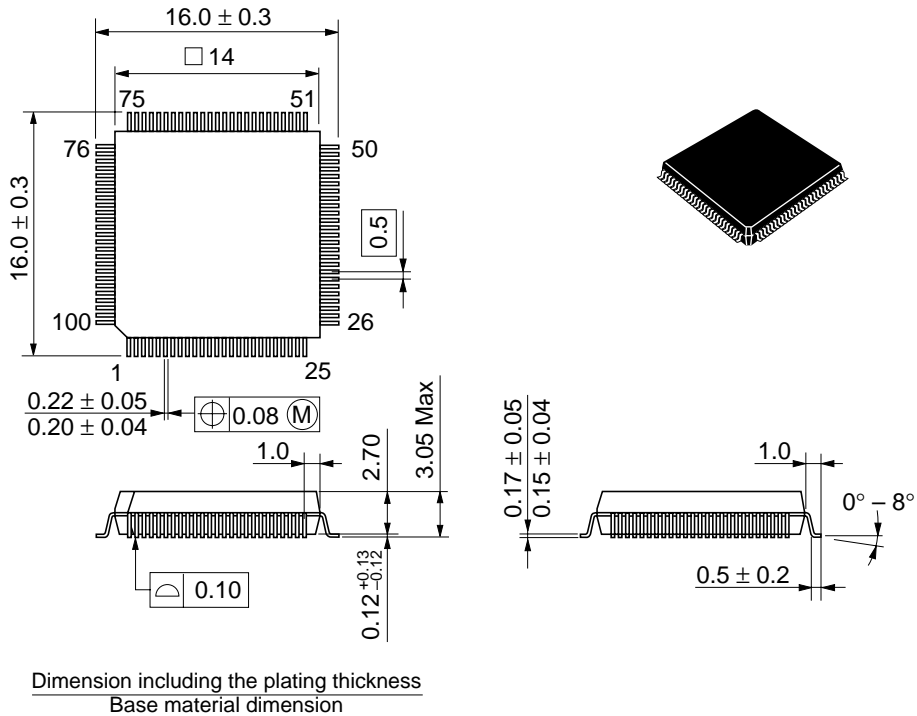
Figure G-1 Package Dimensions (FP-100B)
