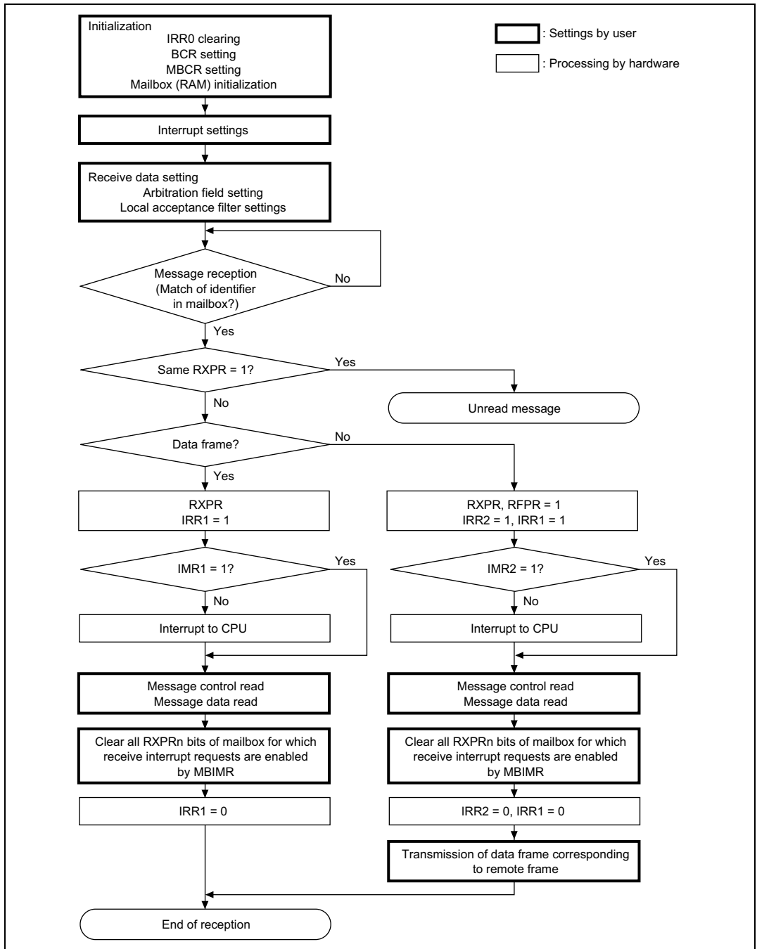
Figure 16-9 Reception Flowchart
