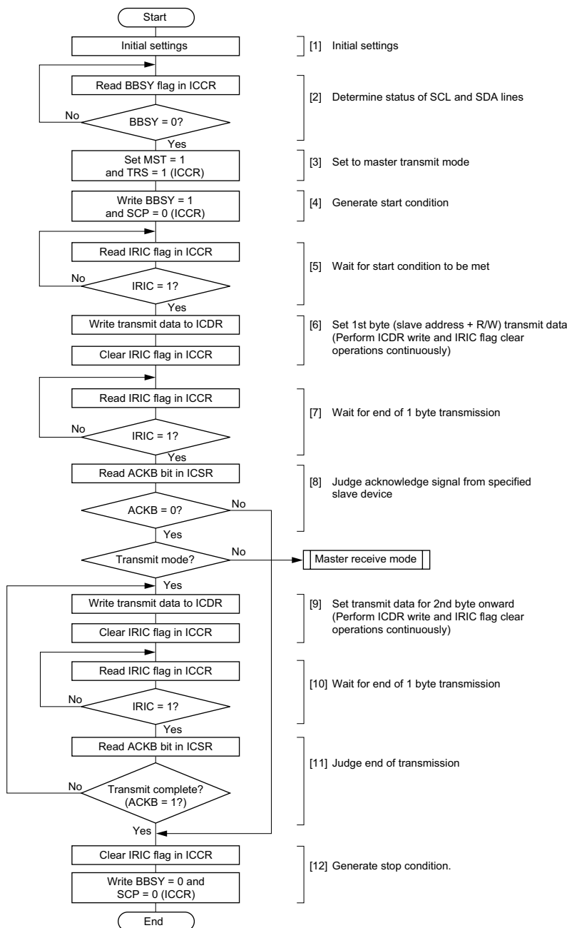
Figure 15-7 Flowchart for Master Transmit Mode (Example)
