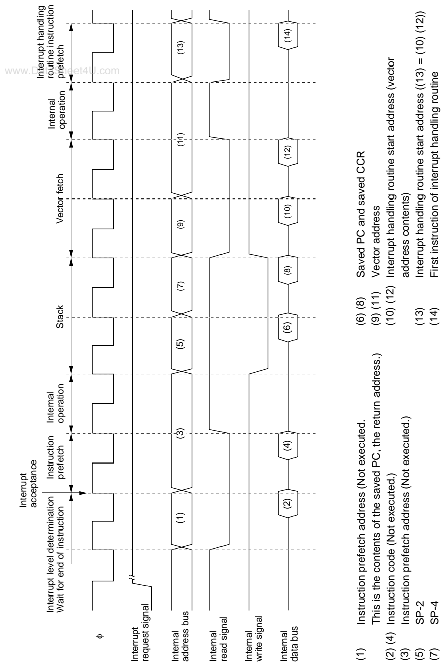
Figure 5.11 Interrupt Exception Handling
