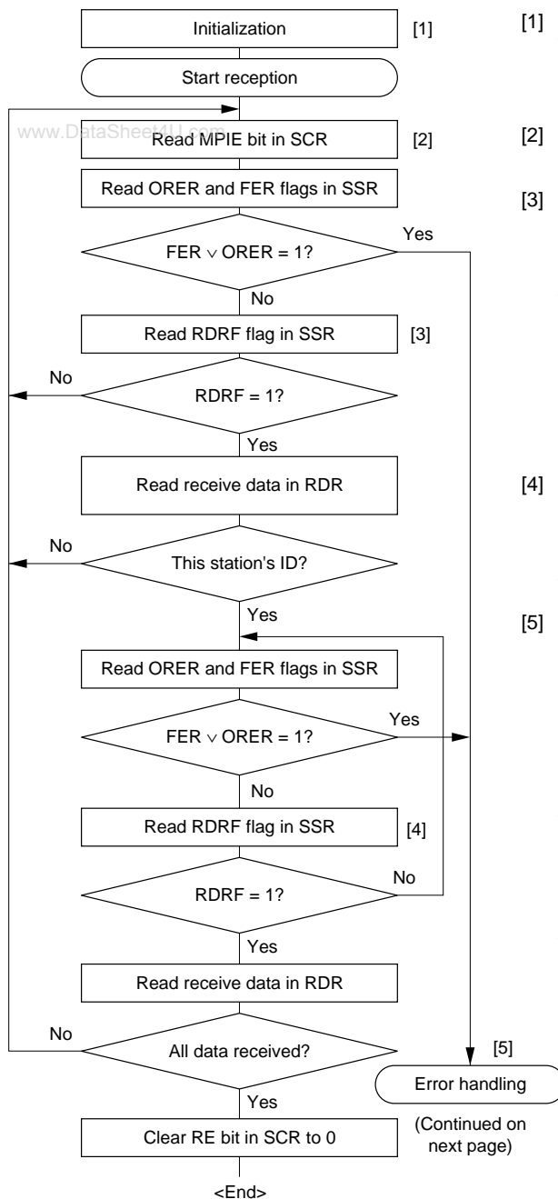
Figure 15.12 Sample Multiprocessor Serial Reception Flowchart
