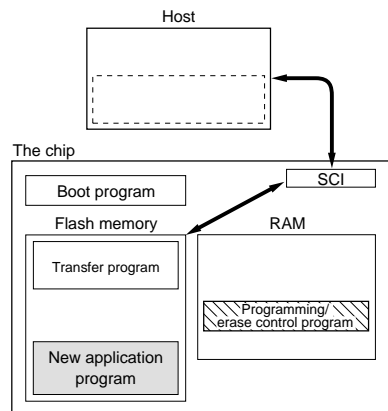
Figure 21.5 User Program Mode (Example)
