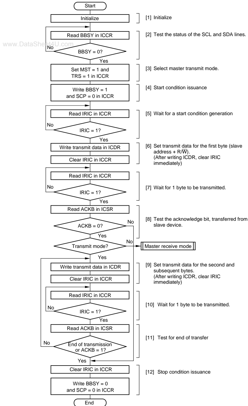
Figure 16.14 Flowchart for Master Transmit Mode (Example)
