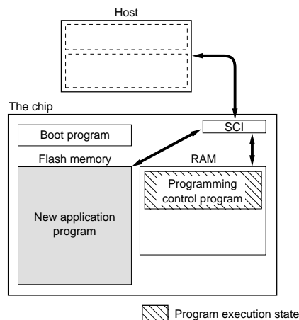
Figure 21.4 Boot Mode
